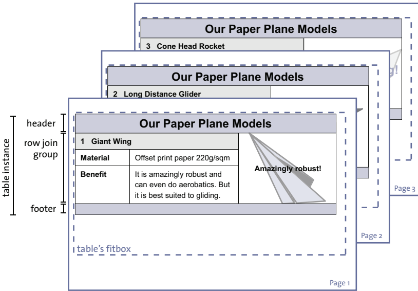
Fig. 8.38 Table broken into several table instances placed in one fitbox each.
