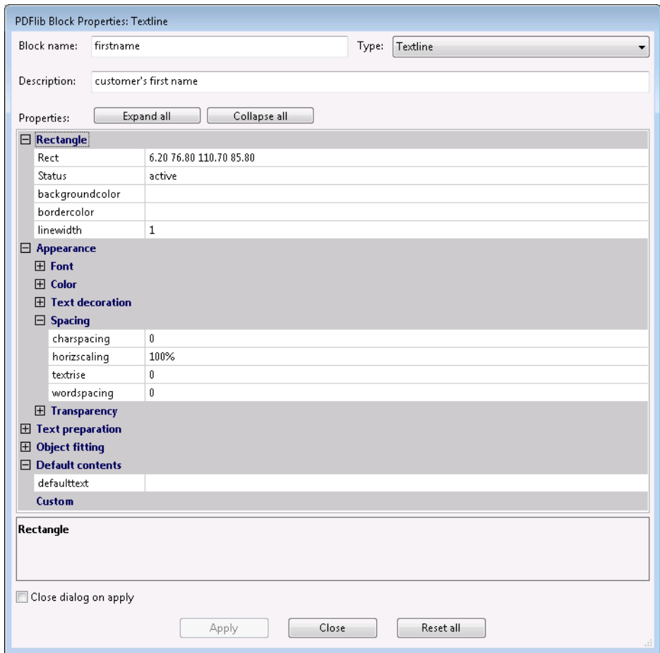
Fig. 12.2 The Block properties dialog
