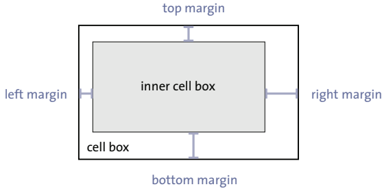
Fig. 8.33 Fitting contents in the inner cell box
